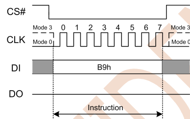
Figure 7.27 Deep Power-down Instruction
