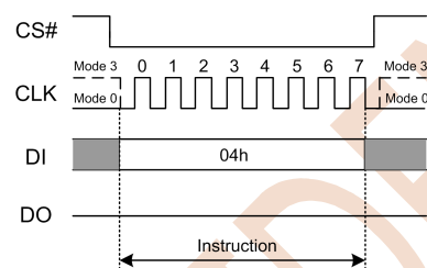
Figure 7.4 Write Disable Instruction
