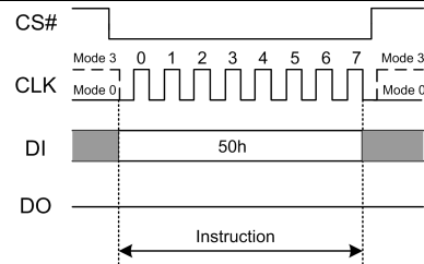
Figure 7.3 Write Enable for Volatile Status Register Instruction
